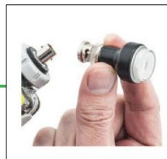
MAC004 strobelight attachment for verifying run speed
